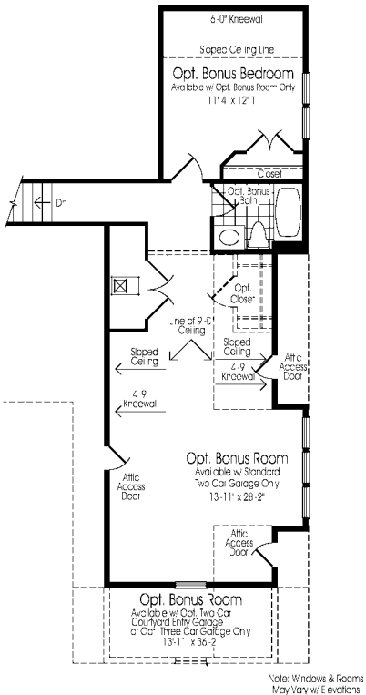
Second Floor w/ Opt. Bonus Room, Opt. Bonus Bedroom & Opt. Bath
