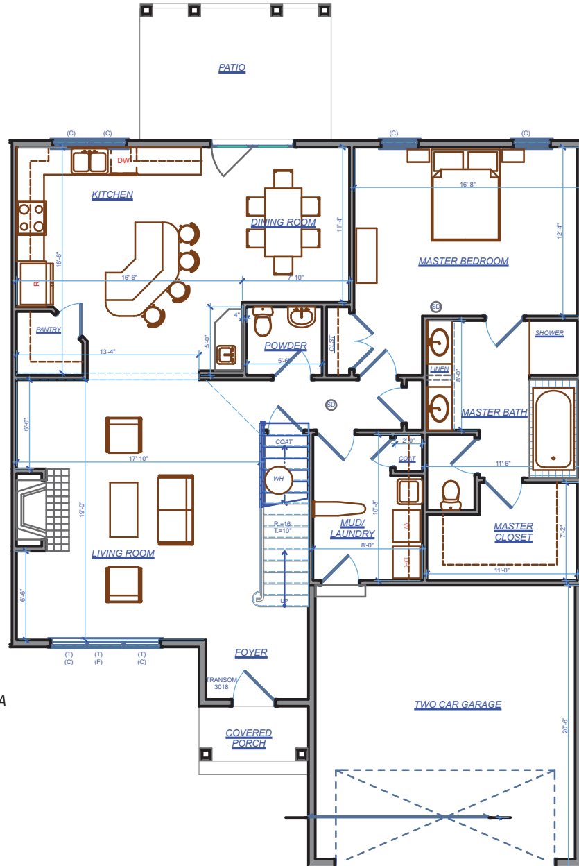
Floor 1
