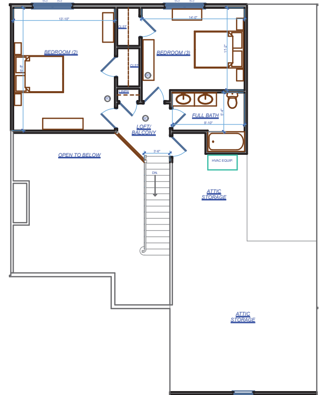
Floor 2
